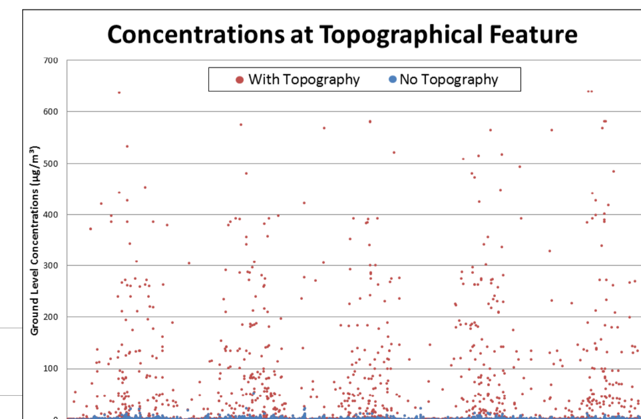
Figure 4. Time series for predicted ground level concentrations at a discrete receptor near the topographical feature.
