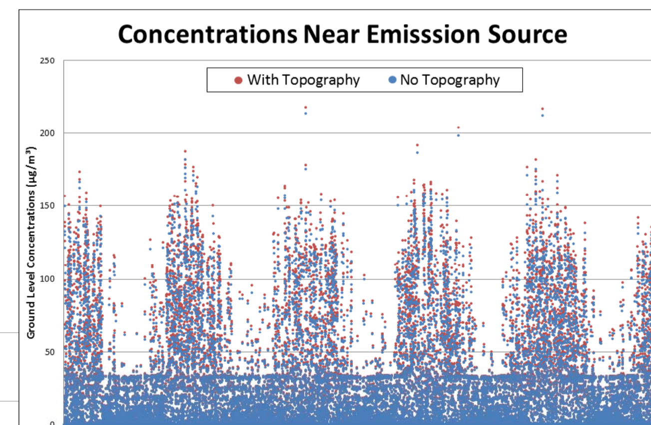
Figure 3. Time series for predicted ground level concentrations at a discrete receptor near the emission source.
